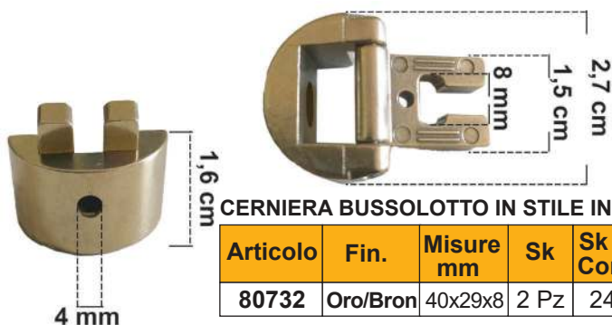
CERNIERA IN STILE IN ZAMA
